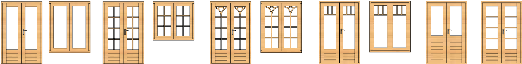
PE45 1210 x 1800 PE45H 1210 x 1935 PE45XL 1510 x 2070 PE44 1210 x 1530 PE24 1210 x 1800 PE24H 1210 x 1935 PE23 1210 x 1140 PE28 1210 x 1800 PE28H 1210 x 1935 PE27 1210 x 1530 PE41 1210 x 1800 PE41H 1210 x 1935 PE40 1210 x 1530 PE60 1210 x 1800 PE60H 1210 x 1935 PE60XL 1510 x 2070 MG02 1210 x 1800 MG02H 1210 x 1935 (melkglas)
